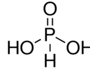
acide Phosphinique H_3PO_2
